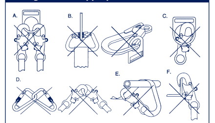
Figure 4 - Inappropriate Connections
