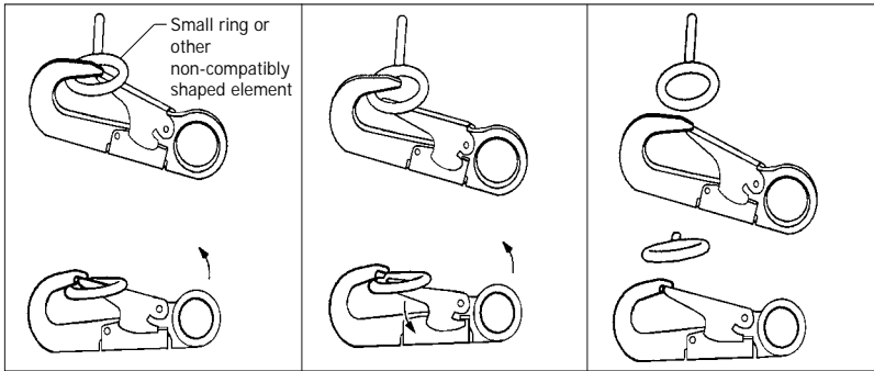
Figure 4 - Inappropriate Connections
